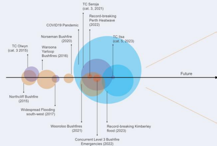
a. Global mean CO 2 concentration and global mean of all greenhouse gas concentrations expressed as CO 2 -e (source: CSIRO and BoM 2022) | b. Anomalies in annual mean sea surface and land temperatures over the Australian region, shown as departures from the 1961-90 standard averaging period (source: CSIRO and BoM 2022) c. see DWER (2021) | d. CSIRO and BoM (2022) | e. timeline of selected emergency events for Western Australia 2015 to present. Circle size represents a qualitative assessment of event magnitude and associated recovery effort.
